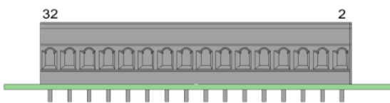
Spring clamp terminals (Max. 12A / terminal)
