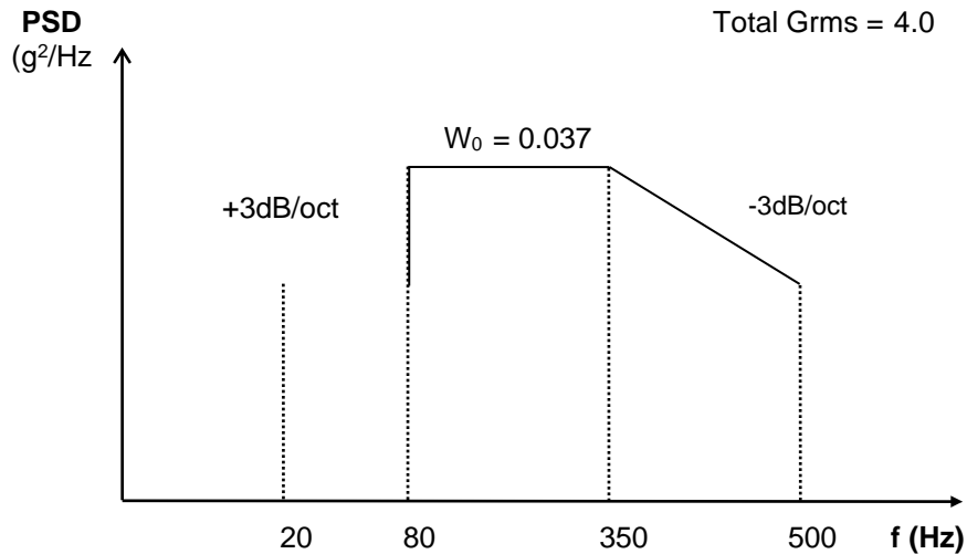
Figure 1 – Vibration Graph
