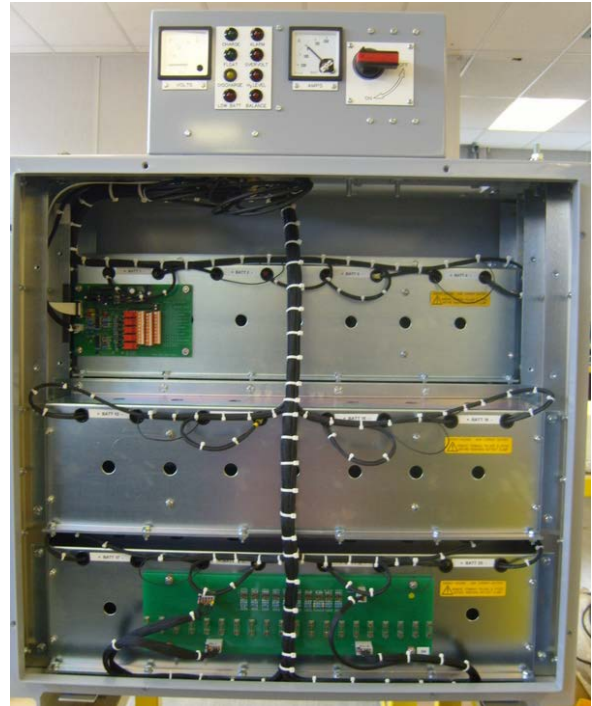
Internal view (battery not fitted)
